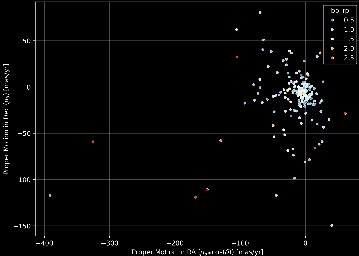
APOGEE DR17 Field: [016+48_MGA] Proper Motion Diagram (n= 192)
