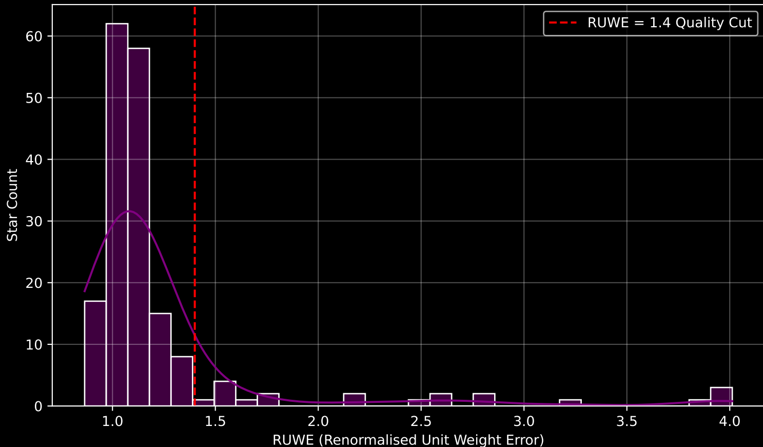
GAPOGEE DR17 Field [016+48_MGA] RUWE Distribution (n= 180)
